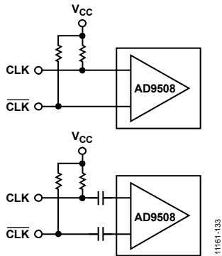
Figure 35. Typical AC-Coupled or DC-Coupled CML Configurations
