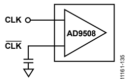
Figure 37. Typical 1.8 V CMOS Configurations for Short Trace Lengths
