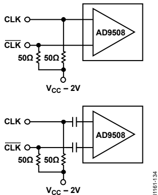
Figure 36. Typical AC-Coupled or DC-Coupled LVPECL Configurations
