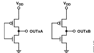
Figure 44. CMOS Equivalent Output Circuit
