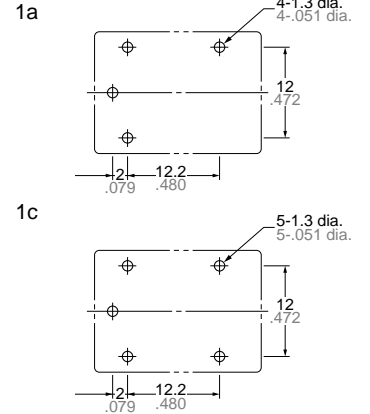
PC board pattern (Copper-side view)
