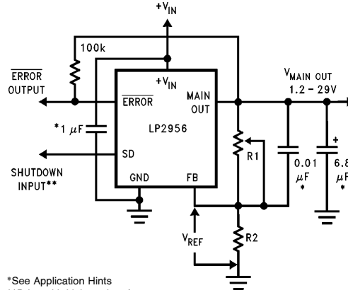
FIGURE 3. Adjustable Regulator
