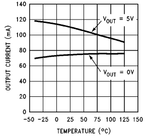
Current Limit vs Temperature (Auxiliary Regulator)
