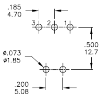
P.C. MOUNTING
